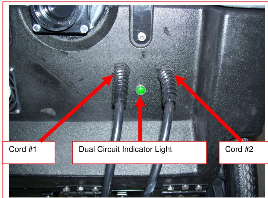
Power Cord – AX32 25' – 12 gauge M-F Plugs
